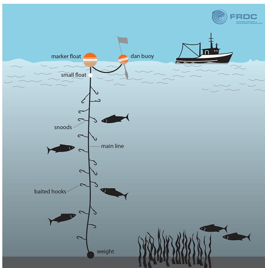
Figure 4. Dropline layout
