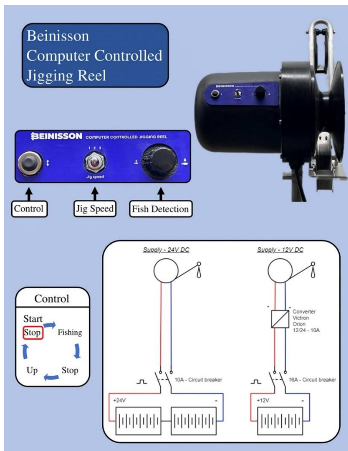
Figure 3. Beinisson Computer Controlled Jigging Reel
