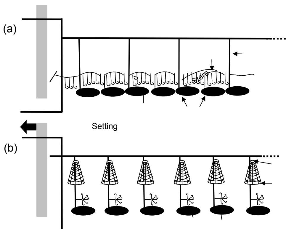
Figure 1. Typical configurations of the traditional Spanish double line system (a) and Chilean (trotline) system (b) showing differences in gear design and location of weights in relation to hooks. The open-ended secondary/connecting lines (not joined by a continuous hook line) and proximity of weights to hooks of the Chilean system enables hooks to sink rapidly and with a linear profile (no lofting in propeller turbulence) from the surface close to vessel sterns. Drawings not to scale.
