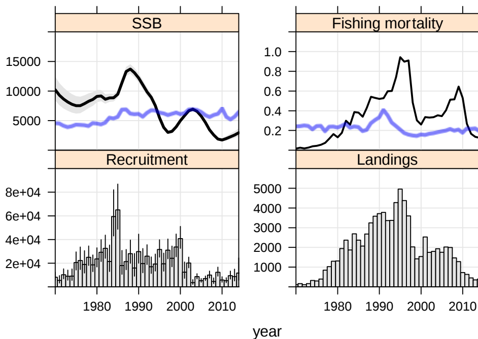
Figure 2. Summary estimates over time showing spawning biomass (kt; top left), recruitment at age 1 (millions; lower left) total fishing mortality (top right) and total catch (kt; bottom right). Blue lines in top figures represent dynamic estimates of F_{MSY} and B_{MSY} for each year (for model 0.4). Confidence bands reflect \pm 1 standard deviation of the estimate.
