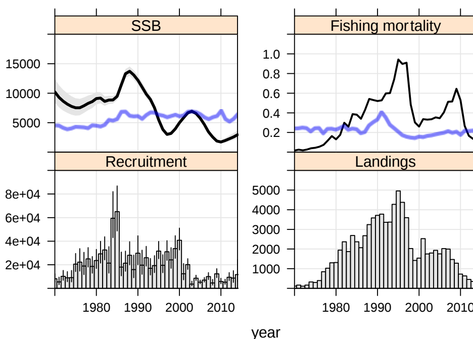
Figure 3. Jack mackerel in the southeast Pacific. Summary of stock assessment. Recruitment (age one) is measured in thousands, catch and SSB in thousands of tonnes, and harvest (fishing mortality) as a rate per year. Note that dynamic values for F_{MSY} and B_{MSY} are shown by horizontal blue lines. Confidence bands reflect \pm 1 standard deviation of the estimate.
