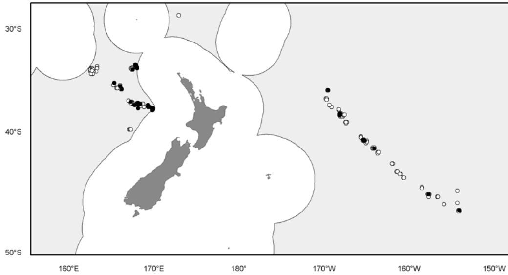
Figure 2. Observed tows (2003-2007) from New Zealand vessels within the SPRFMO area with composite VME score of three or greater based on the 50th percentile thresholds from 1998-2002 (black circles), or tows with score less than 3 (white circles), (N=1010).
