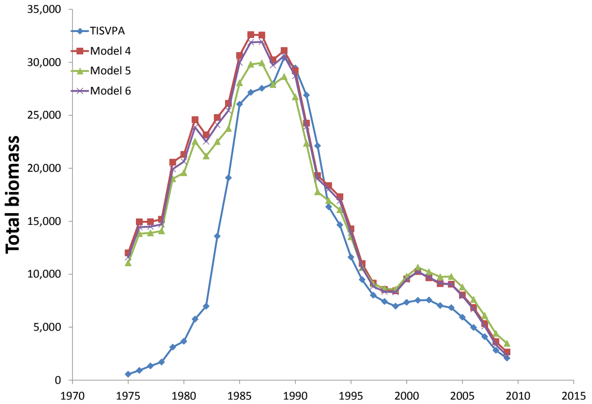
Figure 14. Total biomass estimates comparing the TISVPA model to that of the base case (Model 4) and the two sensitivities that were selected (Models 5 and 6).
