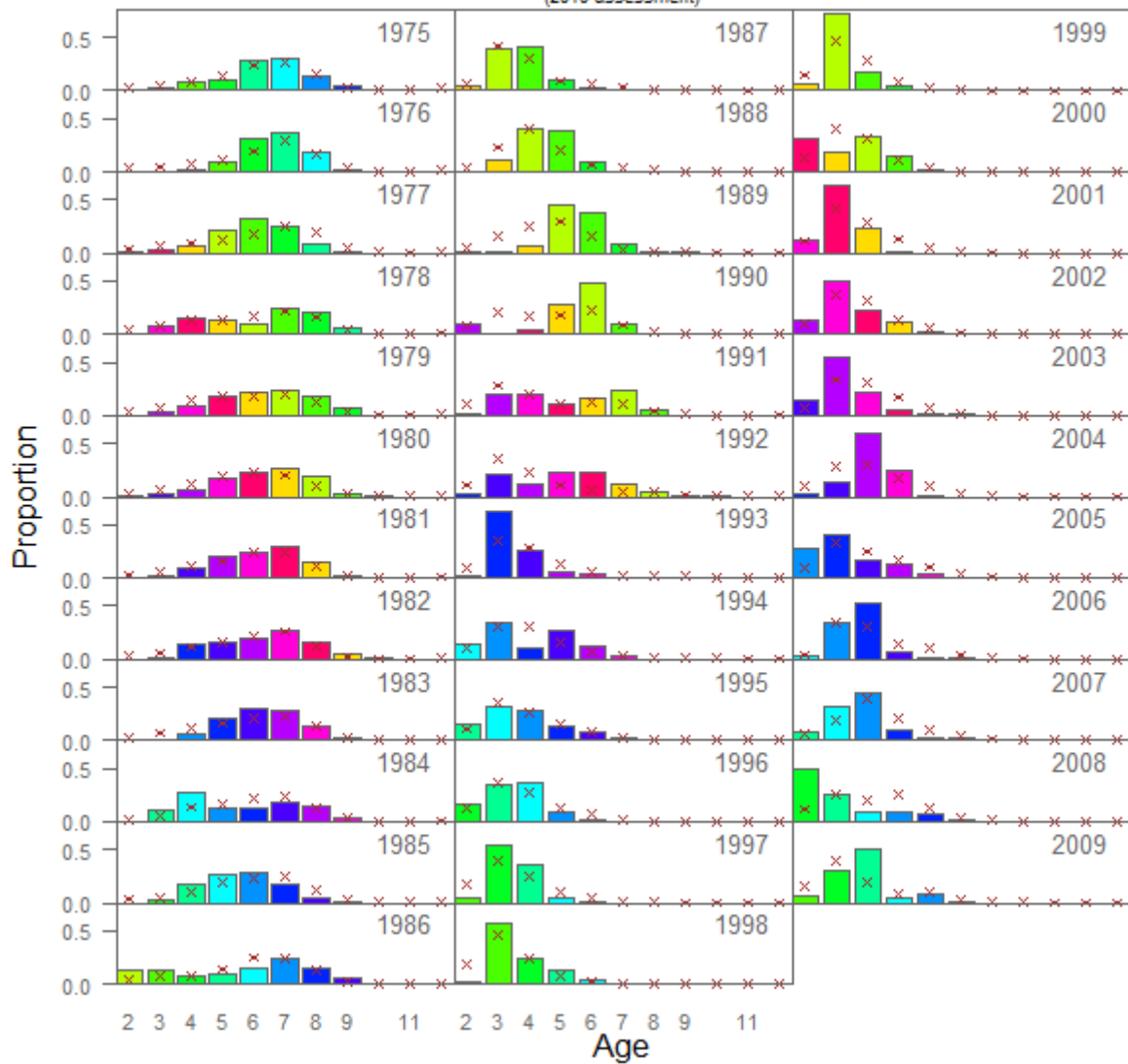
Figure 7. Base case model fit ( x 's) to age composition data (columns) for age samples collected during the CS Chilean region acoustic surveys
