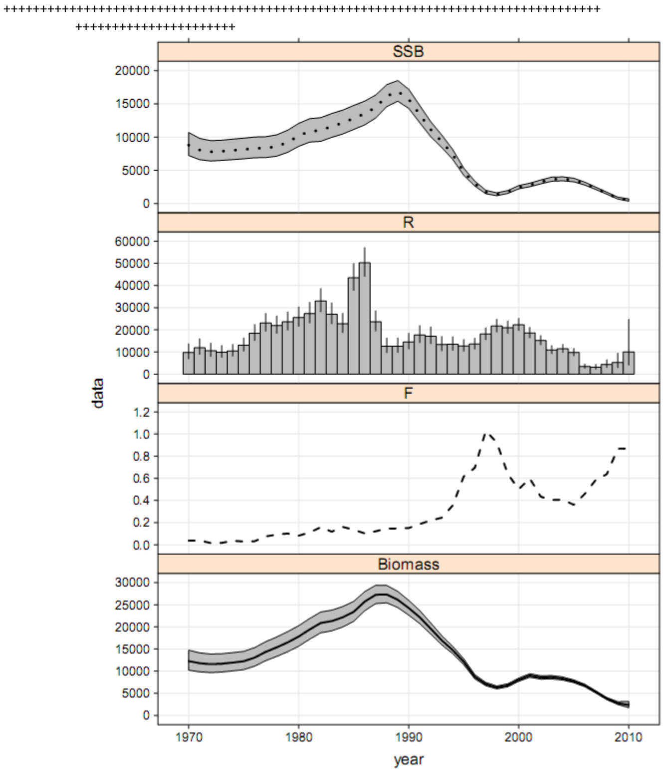
Figure 11. Base case model summary estimates over time showing spawning biomass (kt; top), recruitment at age 2 (millions; 2 nd from top) total fishing mortality (3 rd ) and total biomass (kt; bottom).
