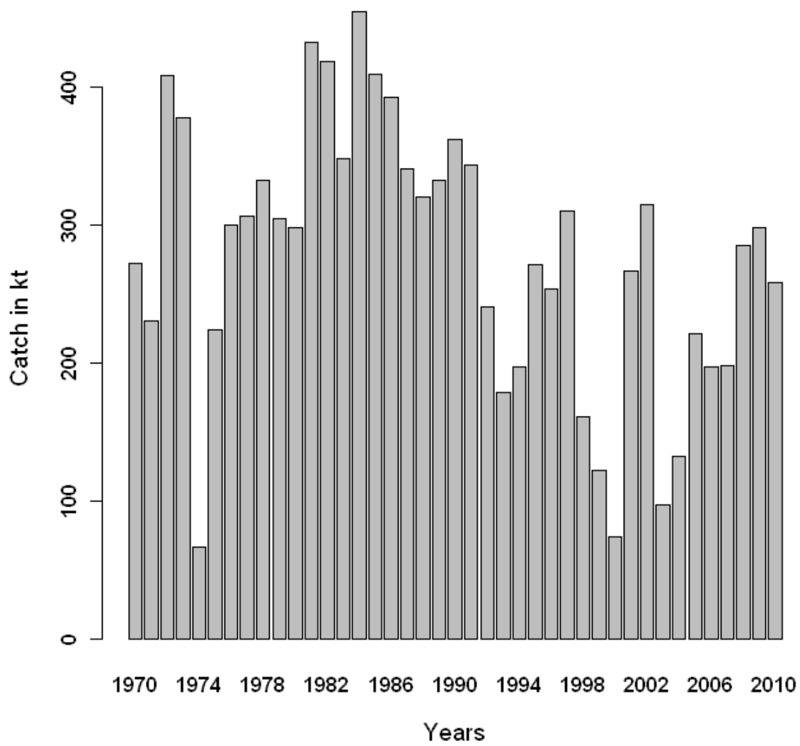
Figure 1. Total catch used for the joint jack mackerel assessment, 1970-2010.
